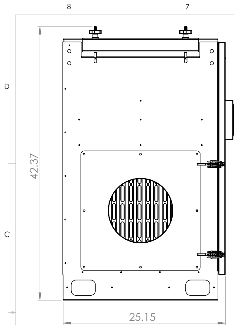
End View
