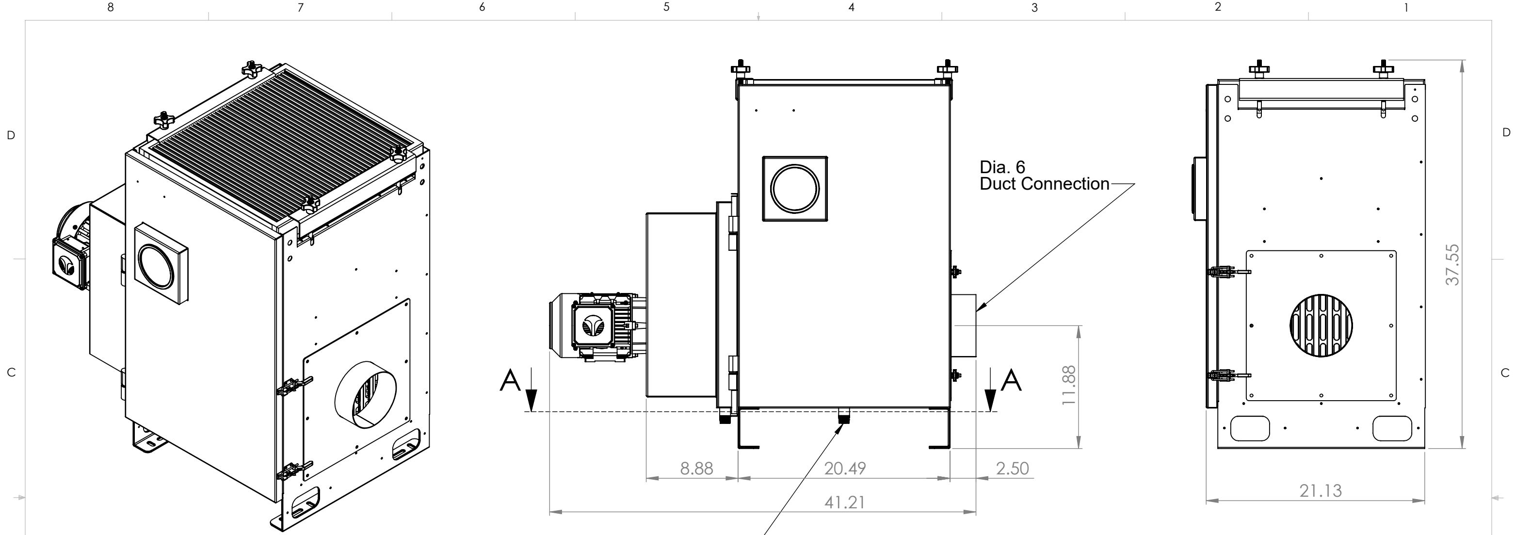
End View
