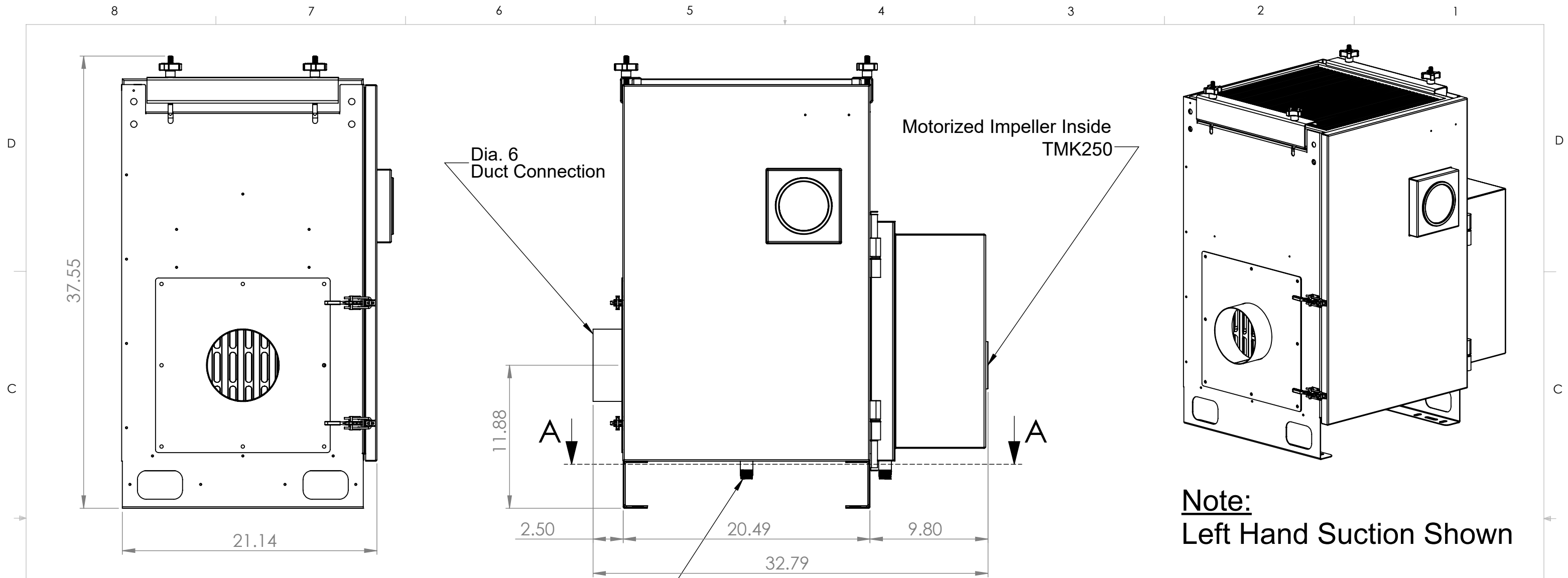
End View
