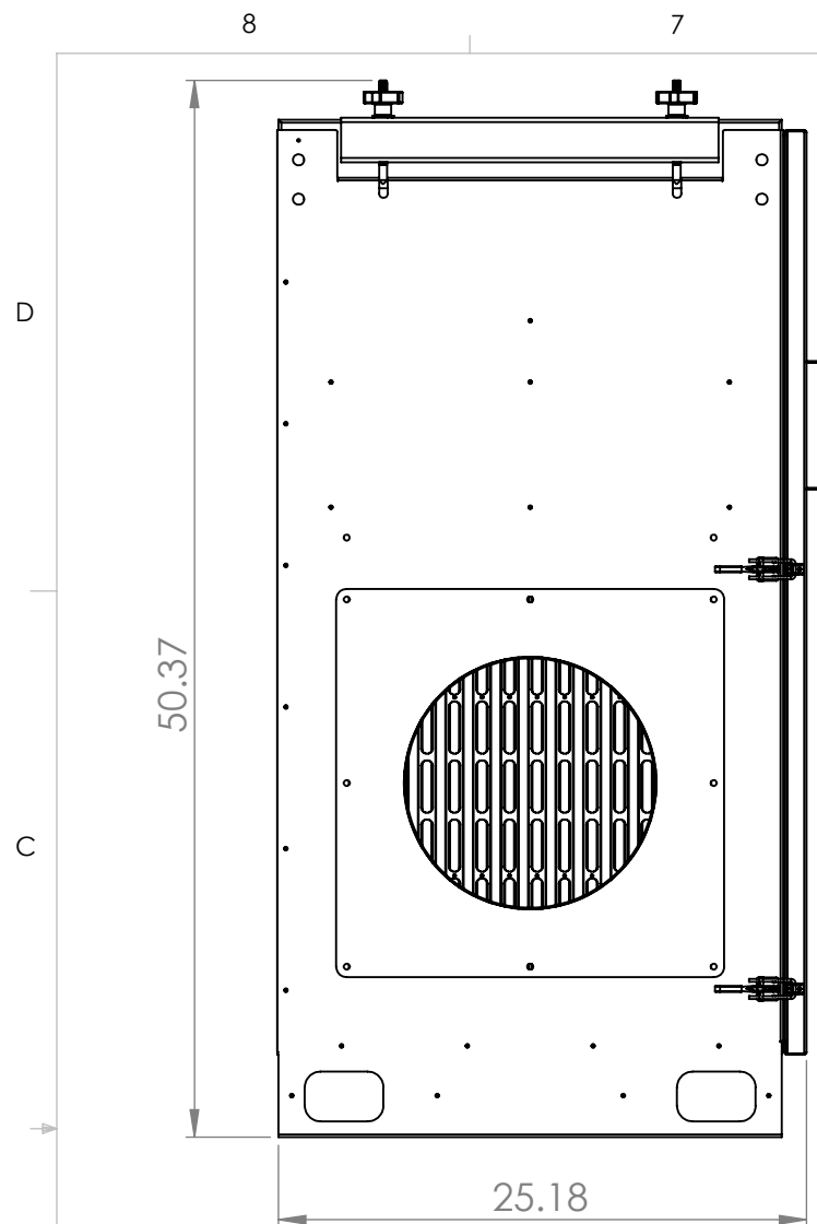
End View
